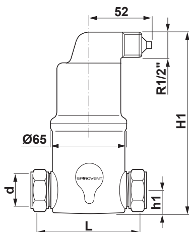
SPIROVENT AA022
